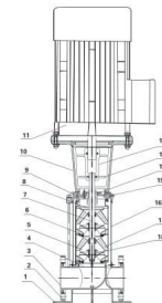
MODEL: LVS120 (150,200)
